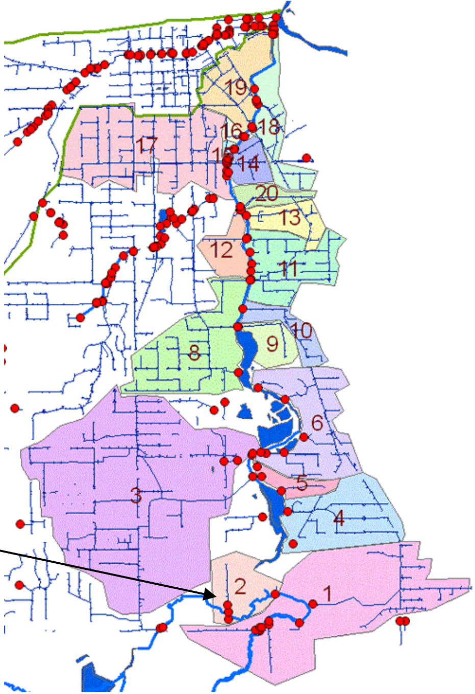
Figure 3-3. Mapped Storm Sewer Drainage Units in the Portage Creek Watershed.
